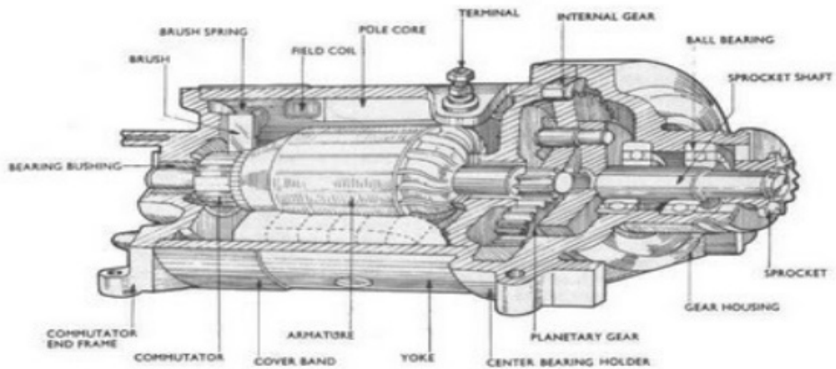
Honda cutaway of 125 starter.
